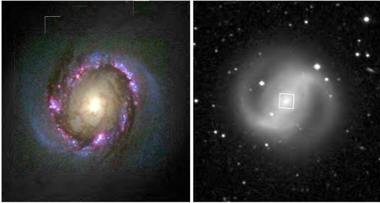
An image from the orbiting Hubble Telescope (left) reveals a ring of baby stars circling galaxy NGC 4314, about 40 million light years away. The baby stars are a blur when seen with a ground-based telescope (right).
